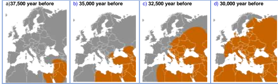
Figure 1: At Cappadocia Homo sapiens, sapiens be there from 35 thousand year before
